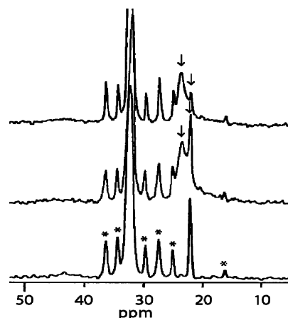
Figure 2. CP-MAS ^{13}\text{C} NMR spectra of 26,27- ^{13}\text{C}_2 ergosterol 4 in the presence and absence of AmB in hydrated POPC membrane at 30 °C. The membrane preparation contained 1/4/POPC at the ratios of 2:1:18 (top), 1:1:9 (middle), and 0:1:9 (bottom) in 10 mM HEPES/ \text{D}_2\text{O} (50 wt %) at pH 7.0. Arrows depict signals due to C26/C27 of ergosterol. (*) Signals are due to POPC.
